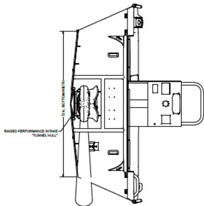
REAR VIEW SCALE 1:12
